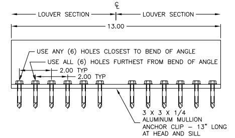
Ⓒ MULLION ANCHOR
